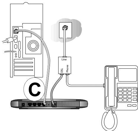
Figure 3-6: Connecting a computer to the DG834G wireless router
