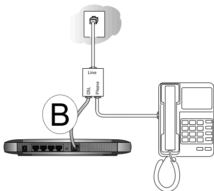
Figure 3-5: Connecting the DG834G wireless router to an ADSL microfilter and phone
